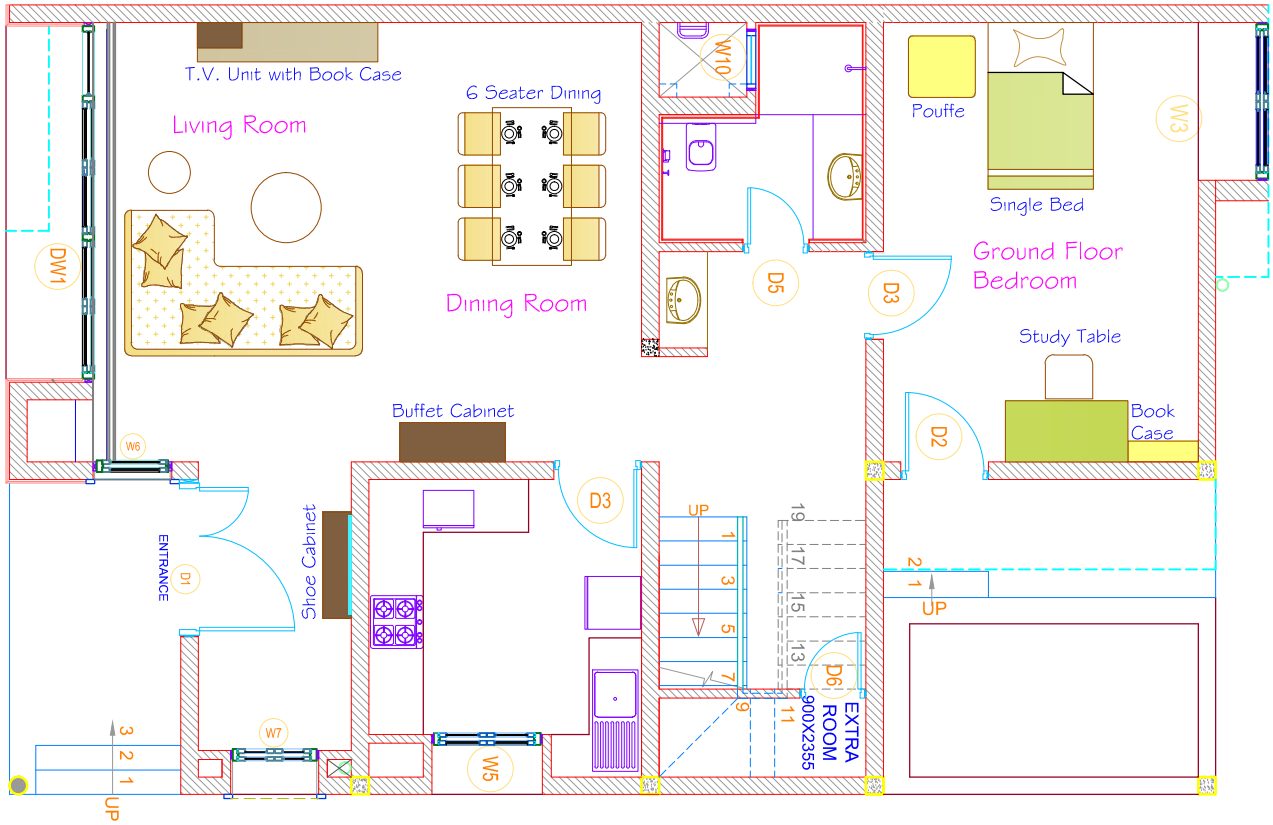
Ground Floor Plan (option 1)
